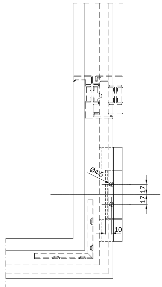
Viti TSP 4.2x13 inox Stainless steel screws TSP 4.2x13
